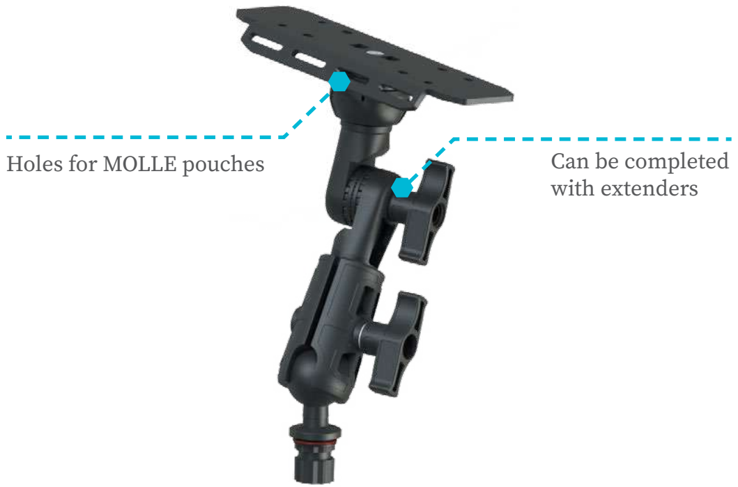
SLr220-3 Tilt plate (AL) for 9" — 12" screen fish finders
